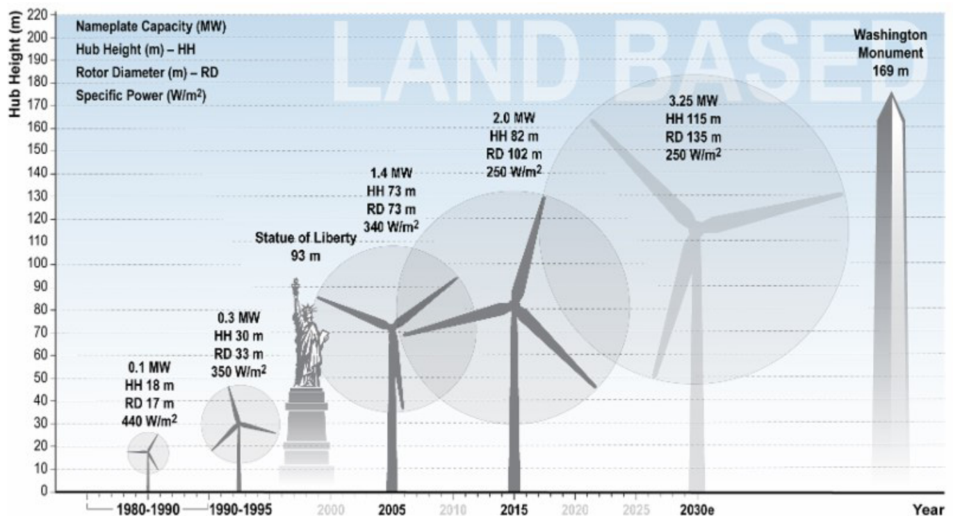
Figure 14. Average Wind Turbine Size and Capacity Is on the Rise
